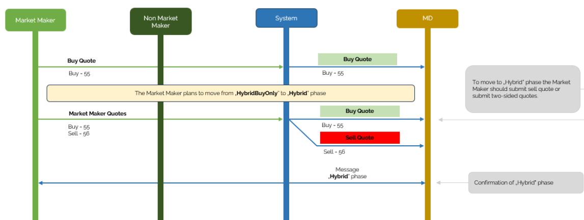
Diagram no 3 - Visualization of the Market Maker changes the trading phase from HybridBuyOnly to Hybrid phase
